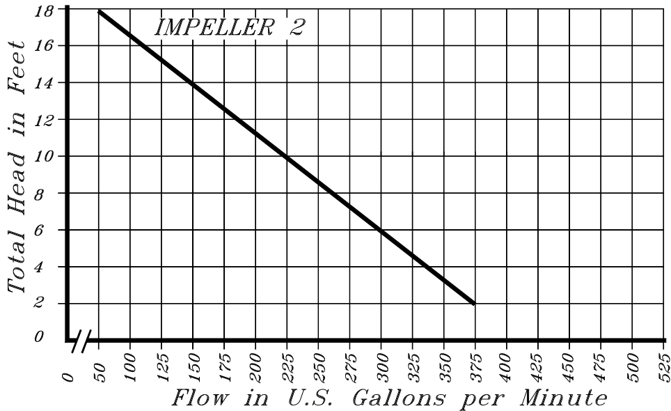
2 HP PERFORMANCE CURVE
