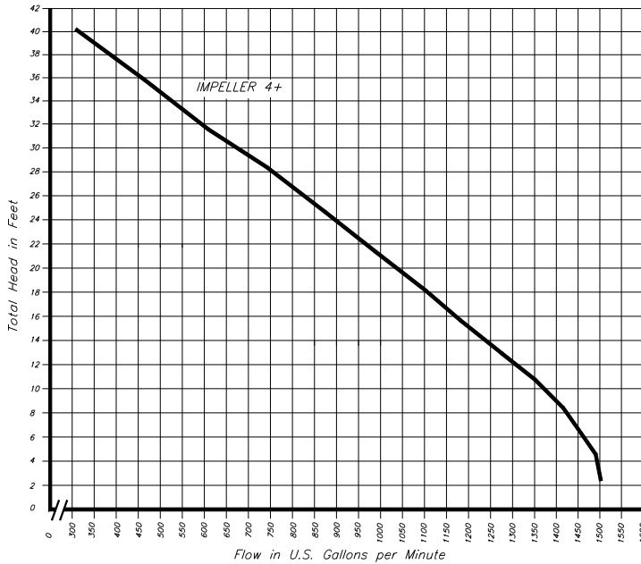
15 HP PERFORMANCE CURVE
